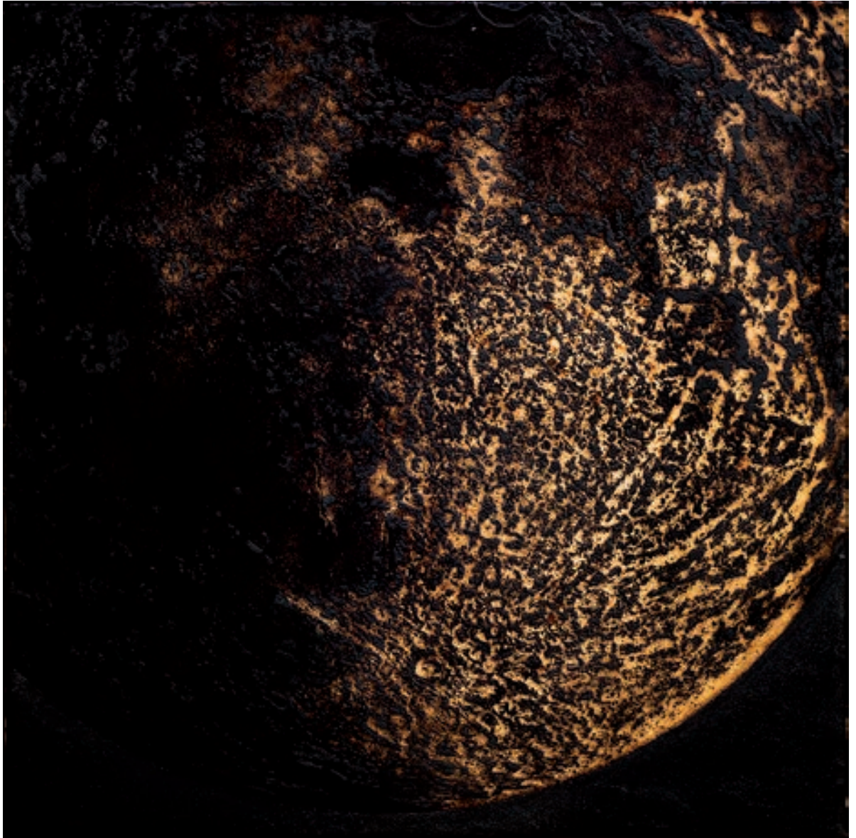
CRATER THYCO
